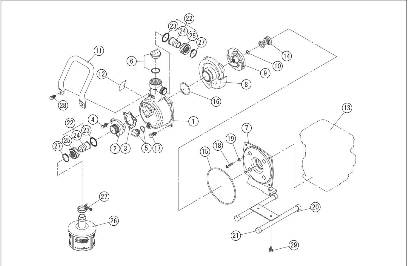
DWG No.012920701 MODELE : SEV-25F FORM : SEV-25F-BAB-0(K35)
